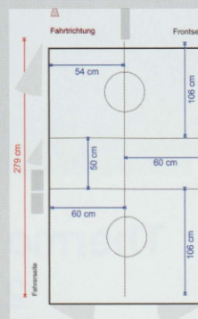
TH 4 Balance Royal Tandemachse double axle
