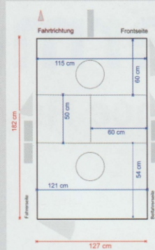
TH 2 Balance Royal 1 Achse single axle
