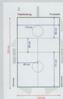
TH 3 Balance Royal Tandemachse double axle
